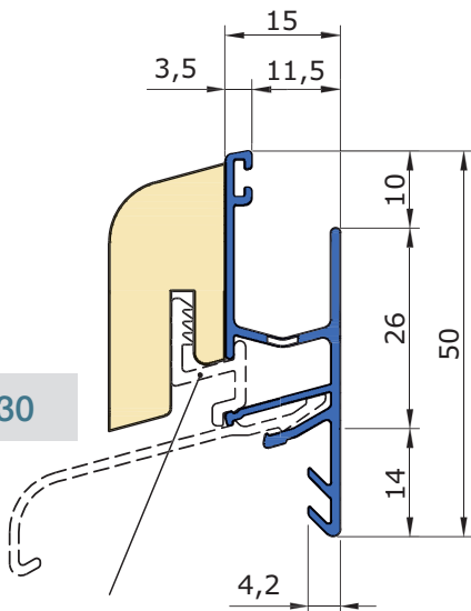
T 3159 (clip L 50 mm)
